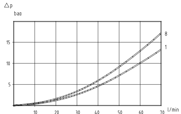
Pressure drop A/B - T, inlet I06B, outlet U01B
