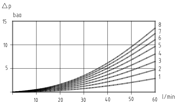
Pressure drop, P1 - T1, inlet I06B, outlet U01B
